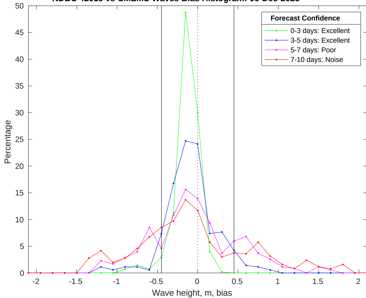
NDBC 42019 vs CMEMS Waves Bias Histogram: 06-Dec-2025
