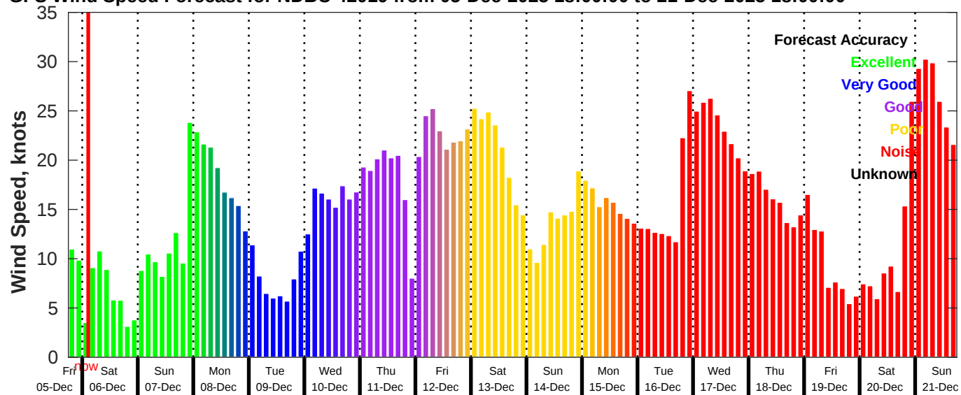
GFS Wind Speed Forecast for NDBC 42019 from 05-Dec-2025 18:00:00 to 21-Dec-2025 18:00:00
