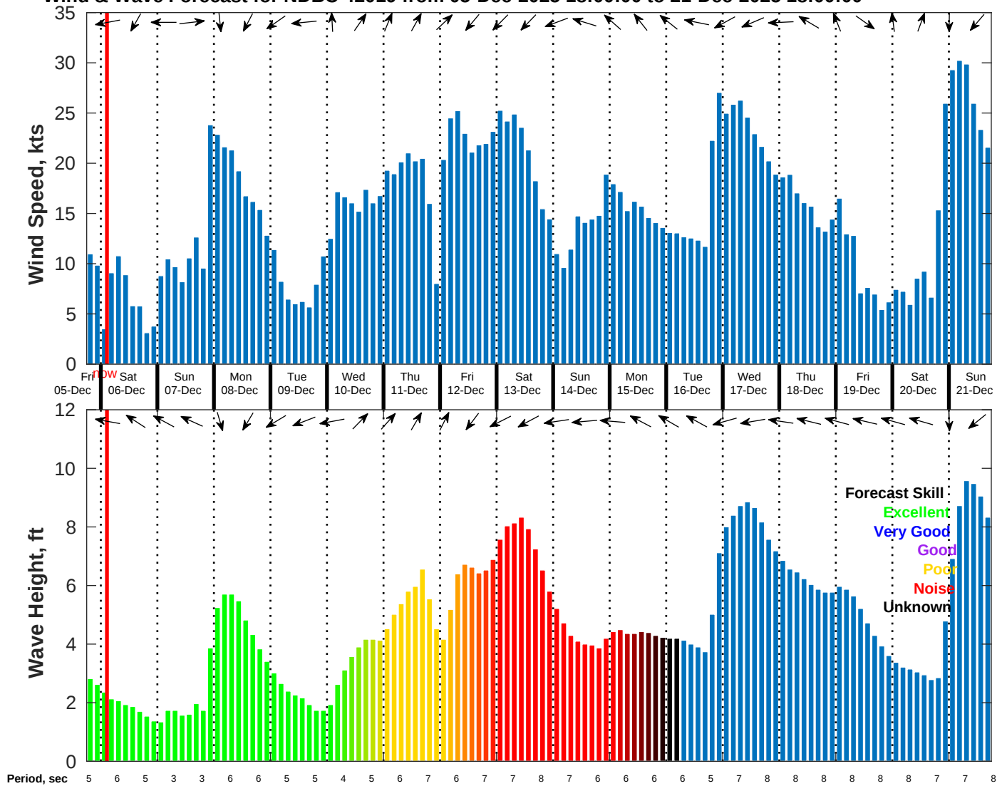
Wind & Wave Forecast for NDBC 42019 from 05-Dec-2025 18:00:00 to 21-Dec-2025 18:00:00
