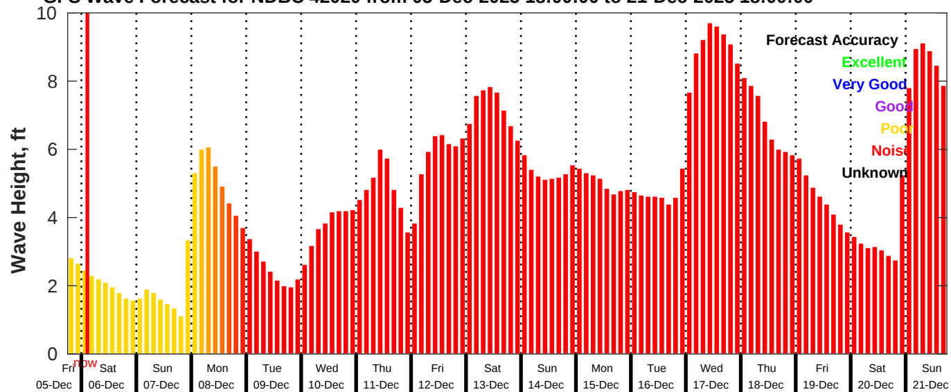
GFS Wave Forecast for NDBC 42020 from 05-Dec-2025 18:00:00 to 21-Dec-2025 18:00:00
