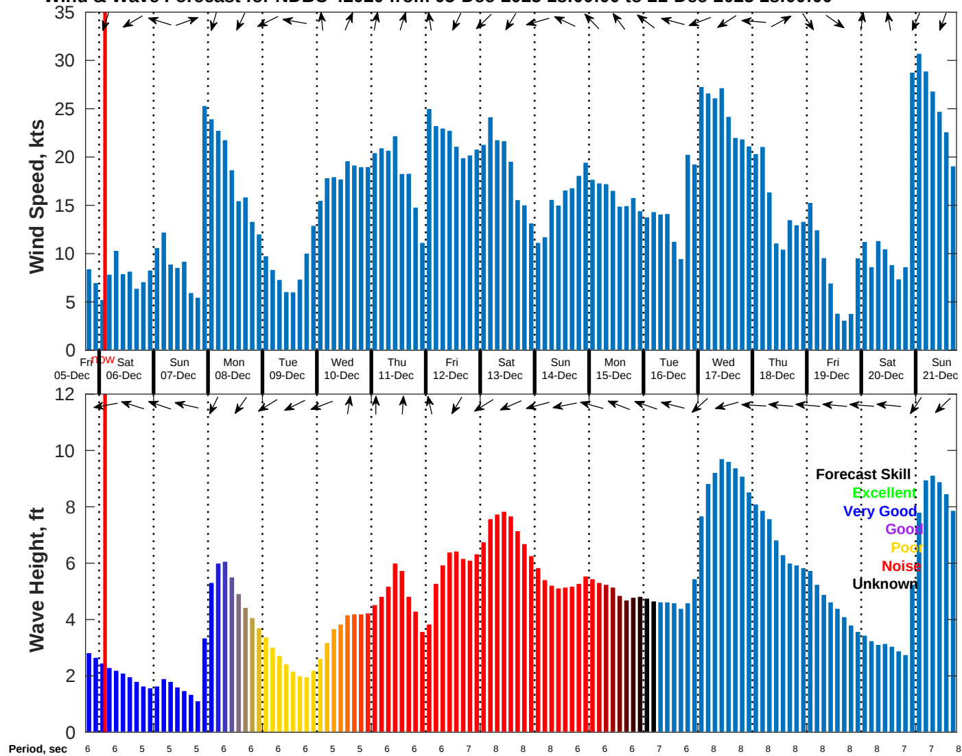
Wind & Wave Forecast for NDBC 42020 from 05-Dec-2025 18:00:00 to 21-Dec-2025 18:00:00
