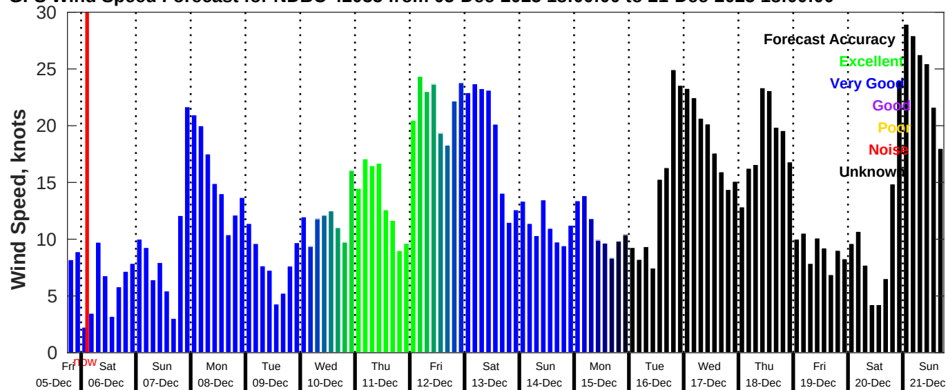
GFS Wind Speed Forecast for NDBC 42035 from 05-Dec-2025 18:00:00 to 21-Dec-2025 18:00:00
