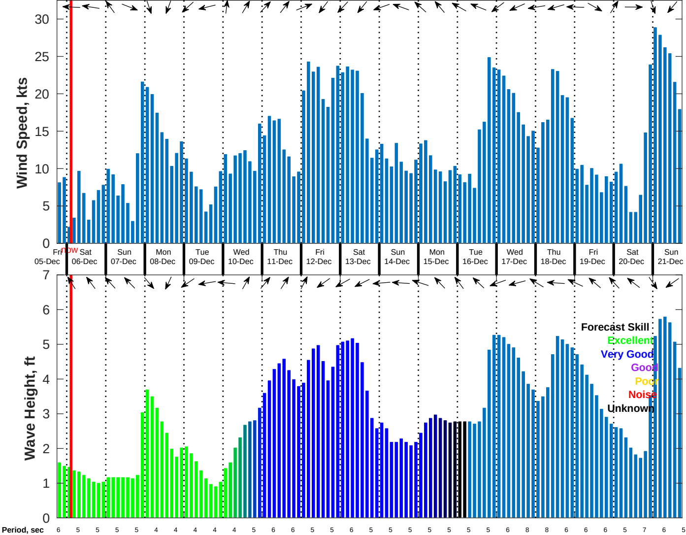
Wind & Wave Forecast for NDBC 42035 from 05-Dec-2025 18:00:00 to 21-Dec-2025 18:00:00
