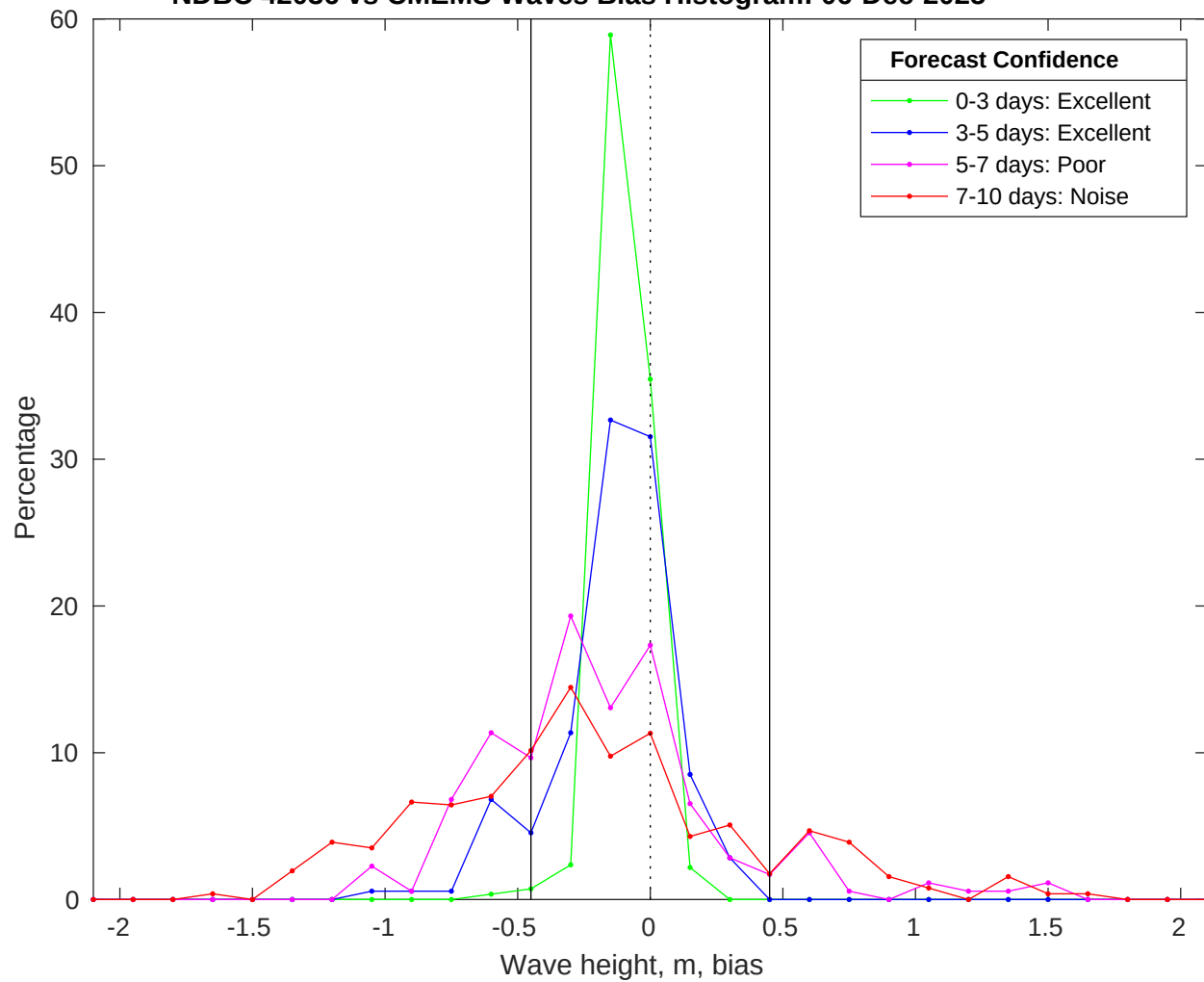
NDBC 42036 vs CMEMS Waves Bias Histogram: 06-Dec-2025
