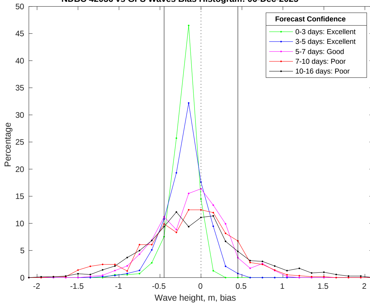
NDBC 42036 vs GFS Waves Bias Histogram: 06-Dec-2025
