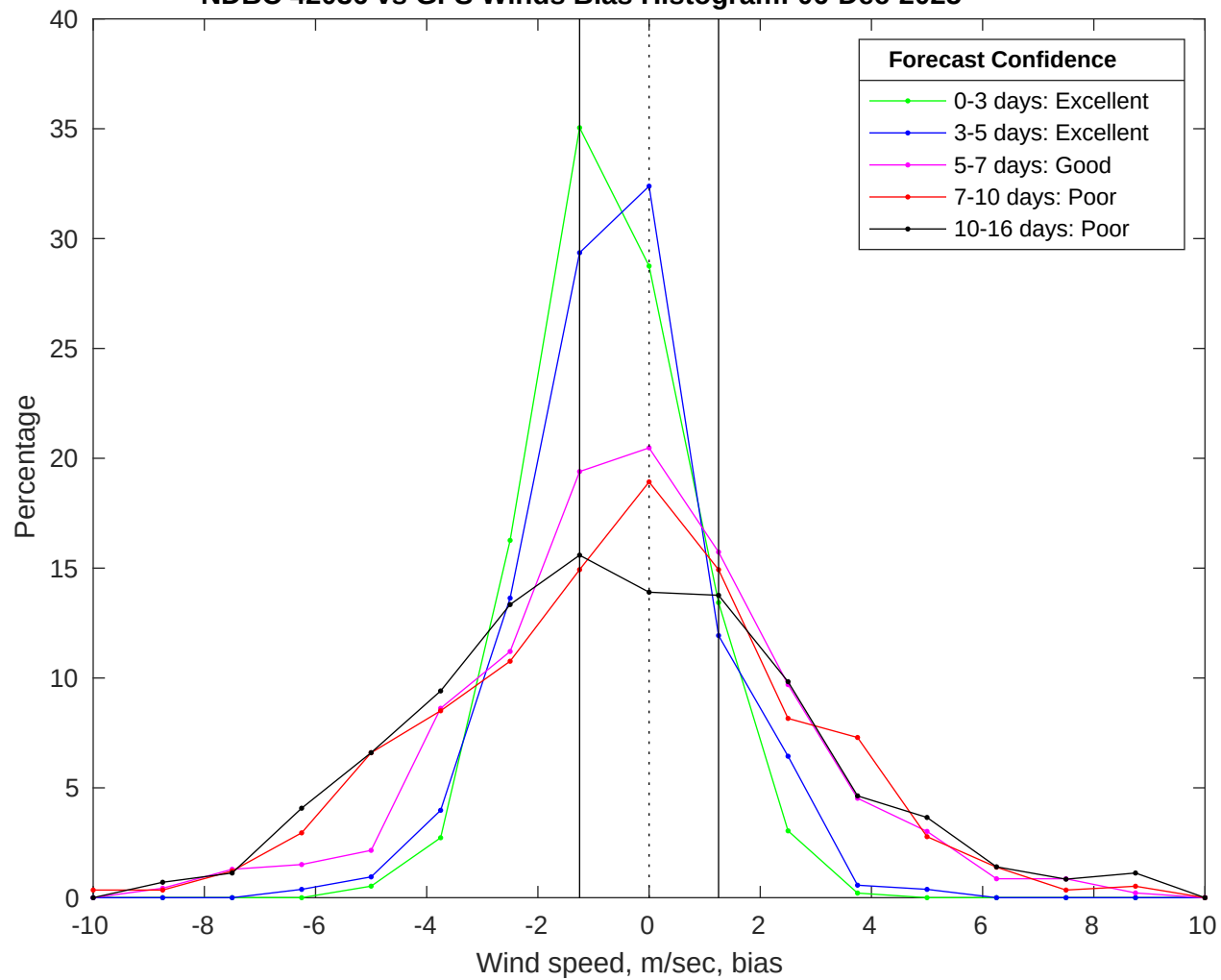
NDBC 42036 vs GFS Winds Bias Histogram: 06-Dec-2025
