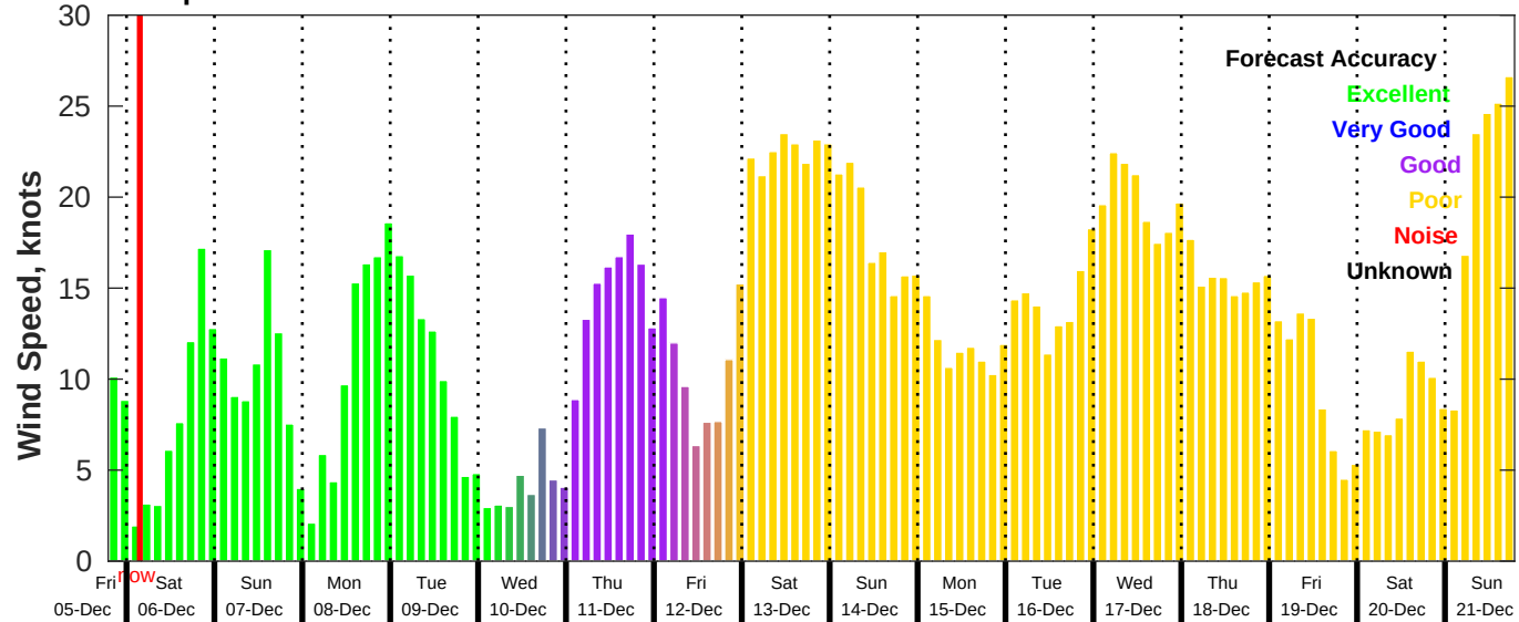
GFS Wind Speed Forecast for NDBC 42036 from 05-Dec-2025 19:00:00 to 21-Dec-2025 19:00:00
