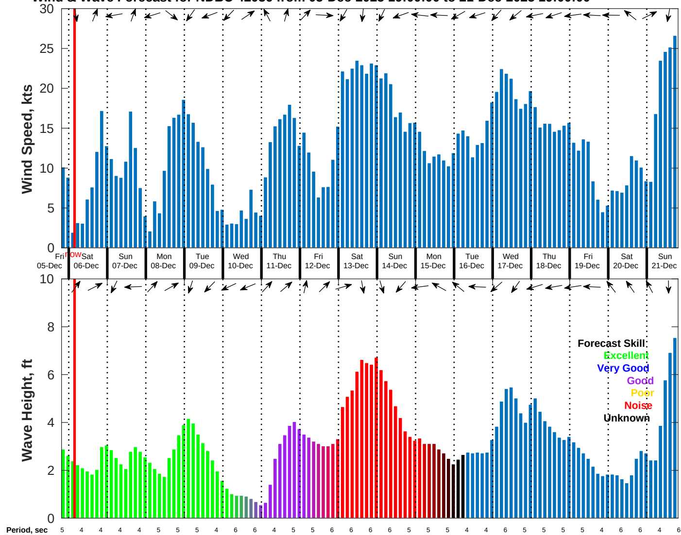
Wind & Wave Forecast for NDBC 42036 from 05-Dec-2025 19:00:00 to 21-Dec-2025 19:00:00
