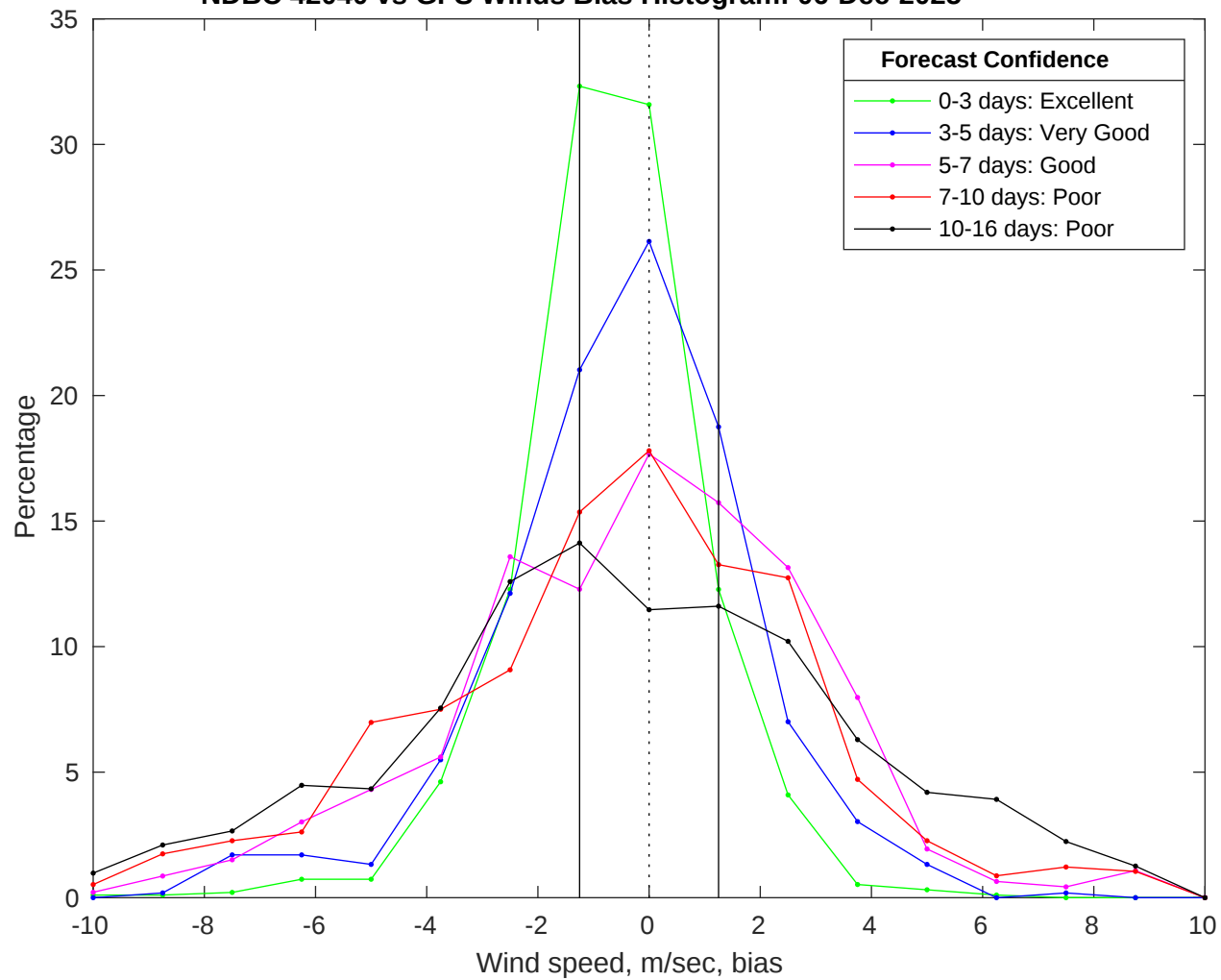
NDBC 42040 vs GFS Winds Bias Histogram: 06-Dec-2025
