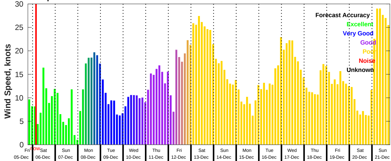
GFS Wind Speed Forecast for NDBC 42040 from 05-Dec-2025 19:00:00 to 21-Dec-2025 19:00:00
