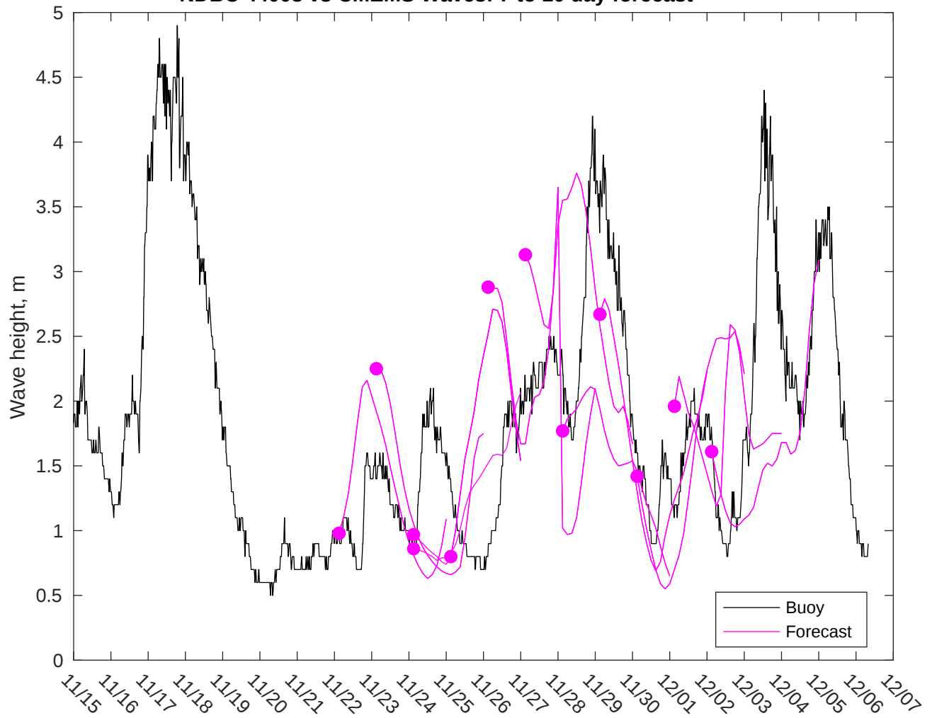
NDBC 44008 vs CMEMS Waves: 7 to 10 day forecast
