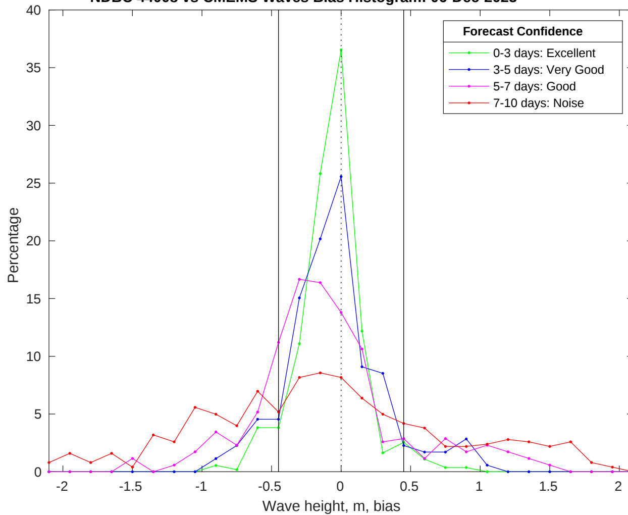
NDBC 44008 vs CMEMS Waves Bias Histogram: 06-Dec-2025
