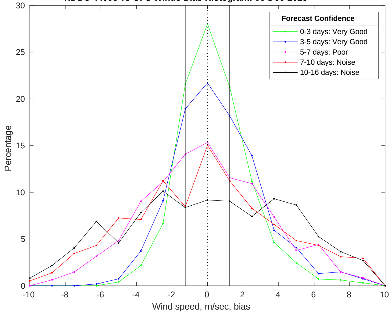
NDBC 44008 vs GFS Winds Bias Histogram: 06-Dec-2025
