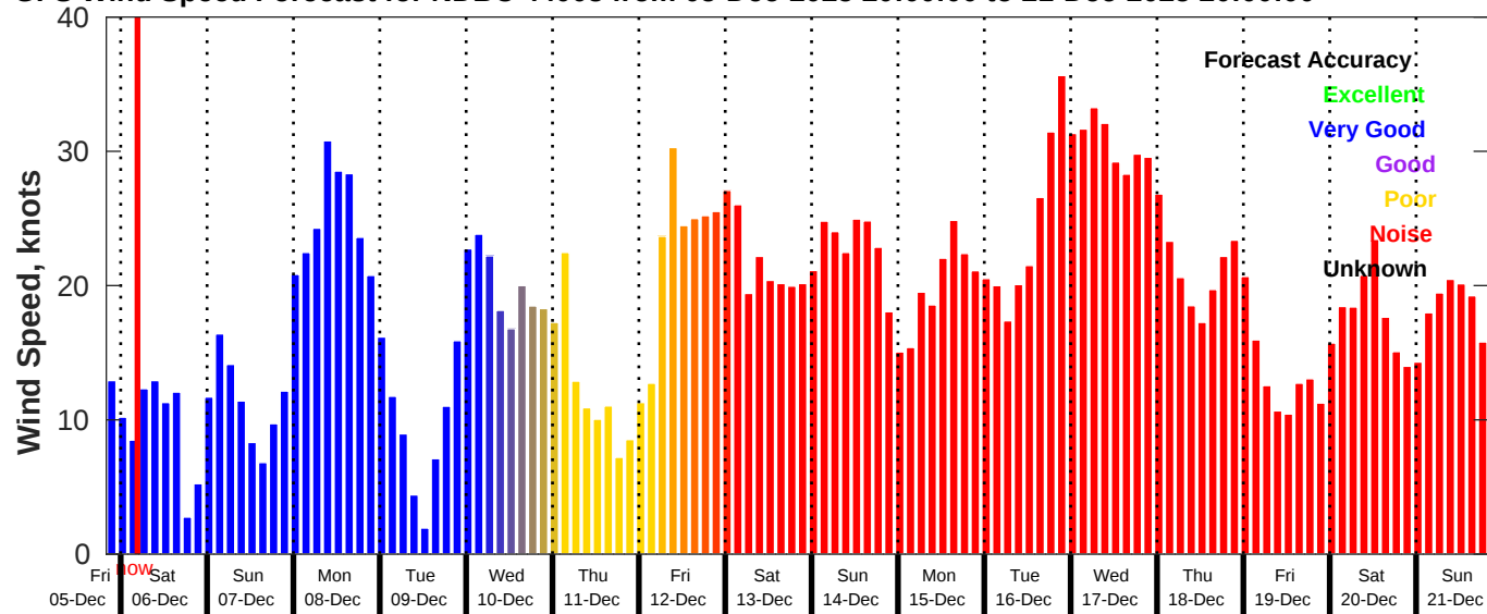
GFS Wind Speed Forecast for NDBC 44008 from 05-Dec-2025 20:00:00 to 21-Dec-2025 20:00:00
