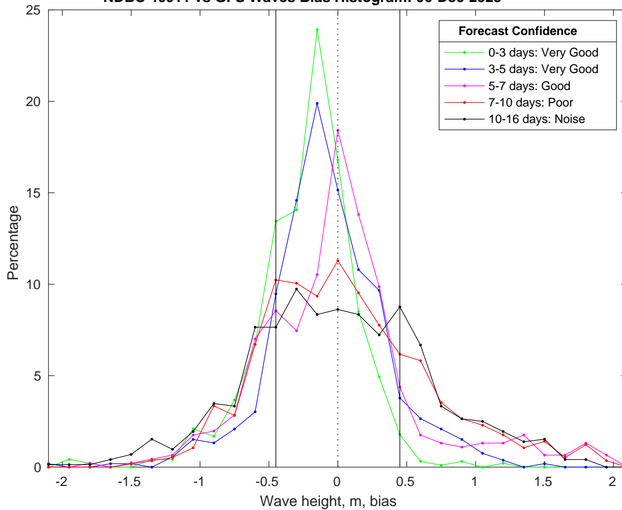
NDBC 46011 vs GFS Waves Bias Histogram: 06-Dec-2025
