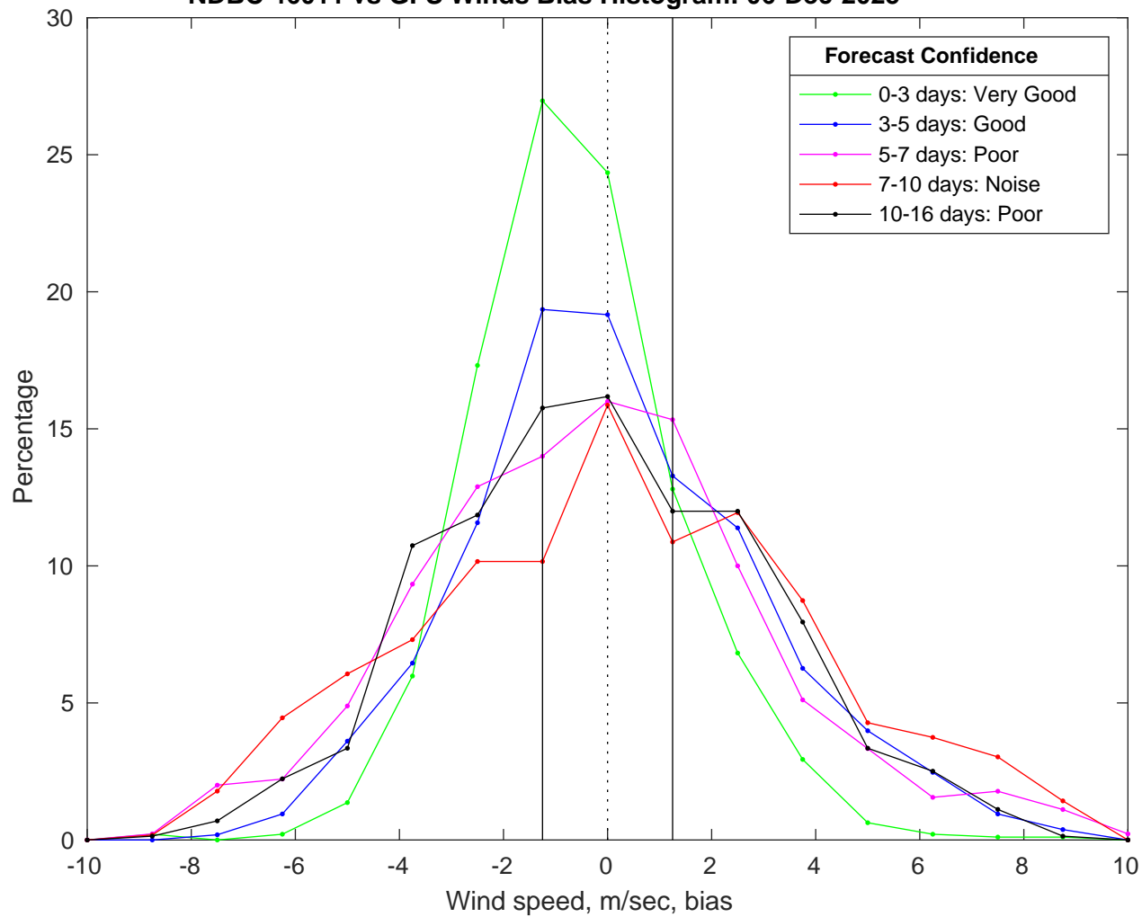
NDBC 46011 vs GFS Winds Bias Histogram: 06-Dec-2025
