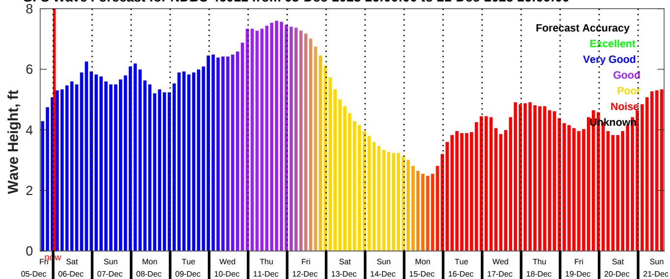
GFS Wave Forecast for NDBC 46011 from 05-Dec-2025 16:00:00 to 21-Dec-2025 16:00:00
