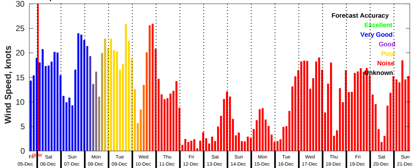
GFS Wind Speed Forecast for NDBC 46028 from 05-Dec-2025 16:00:00 to 21-Dec-2025 16:00:00
