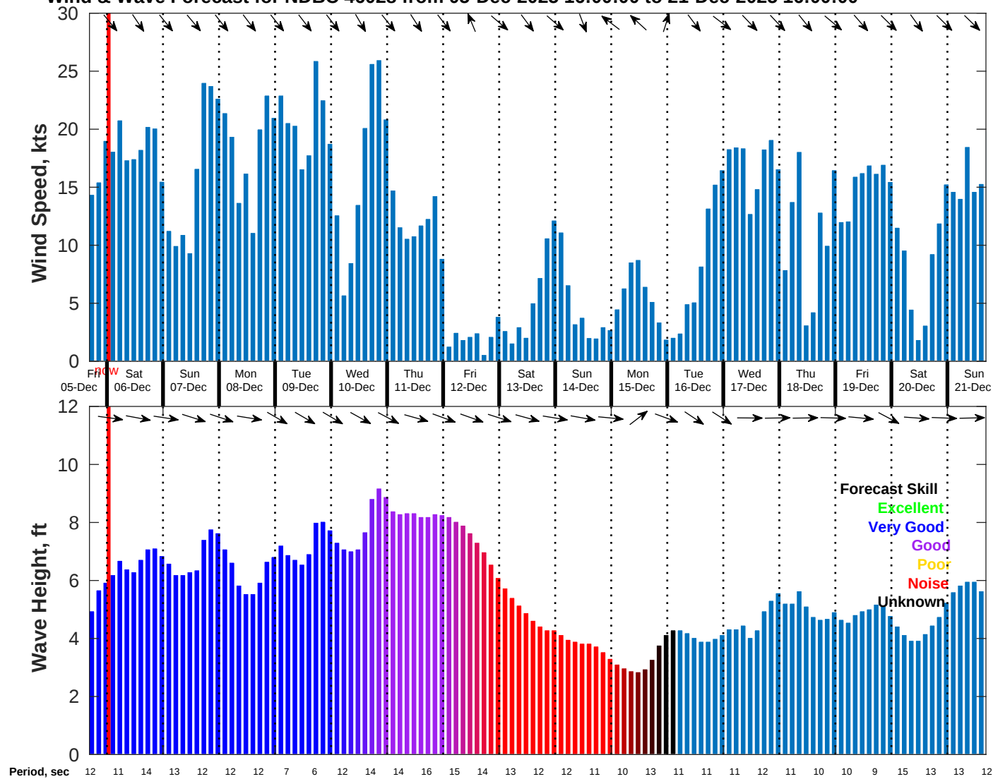
Wind & Wave Forecast for NDBC 46028 from 05-Dec-2025 16:00:00 to 21-Dec-2025 16:00:00
