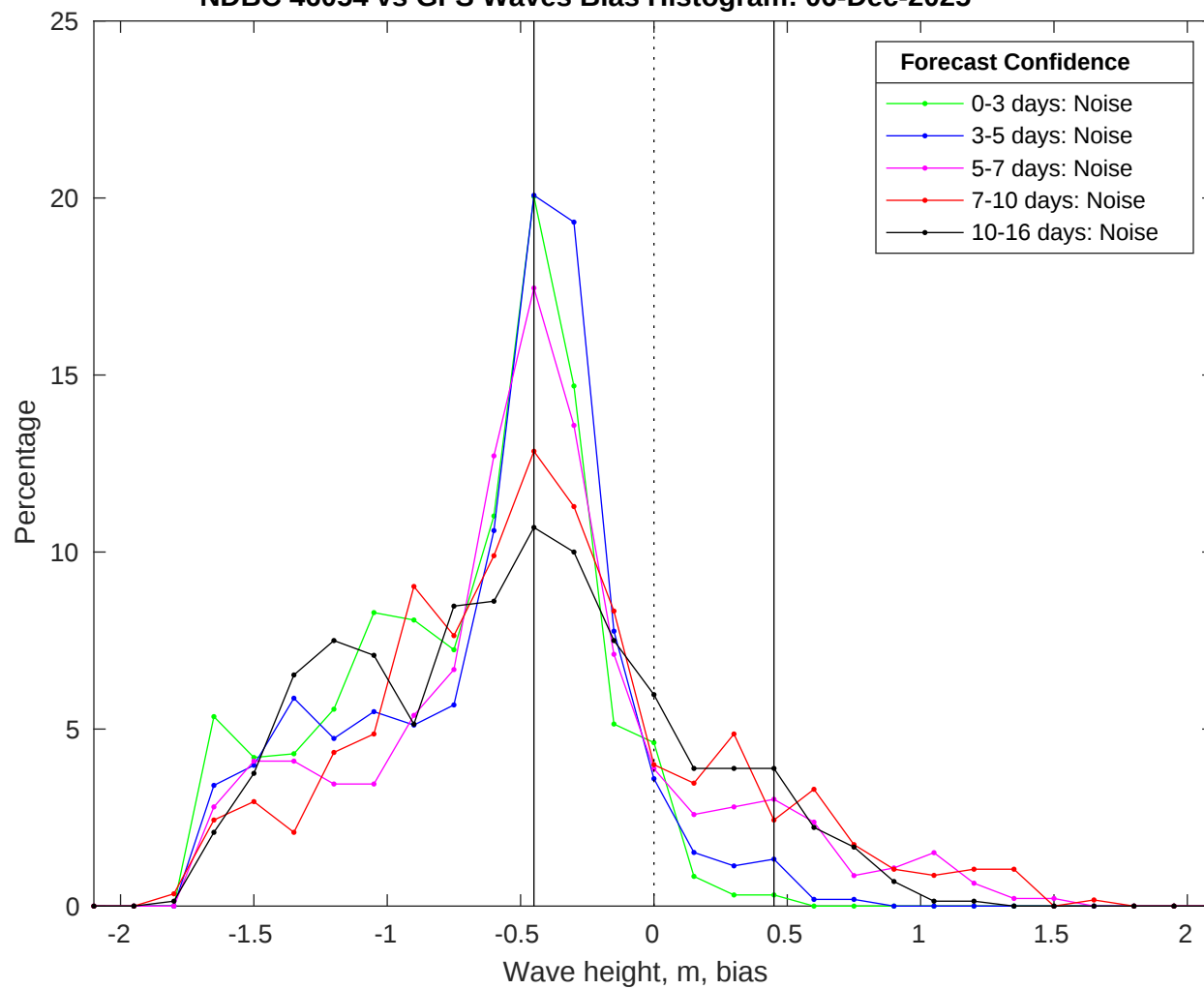
NDBC 46054 vs GFS Waves Bias Histogram: 06-Dec-2025
