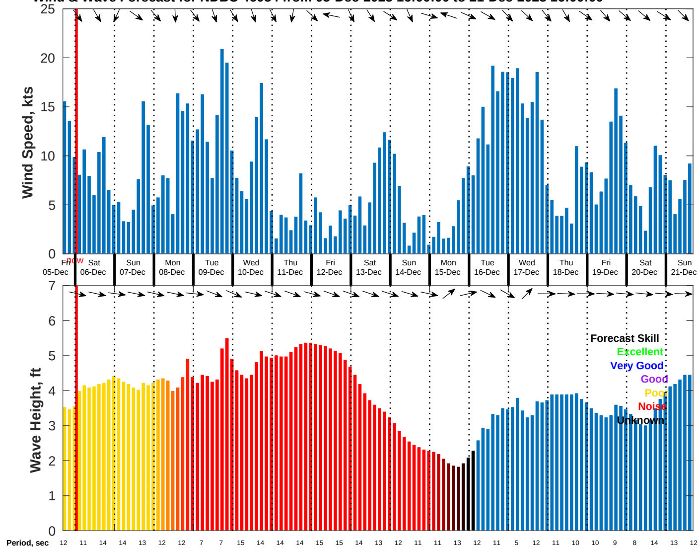
Wind & Wave Forecast for NDBC 46054 from 05-Dec-2025 16:00:00 to 21-Dec-2025 16:00:00
