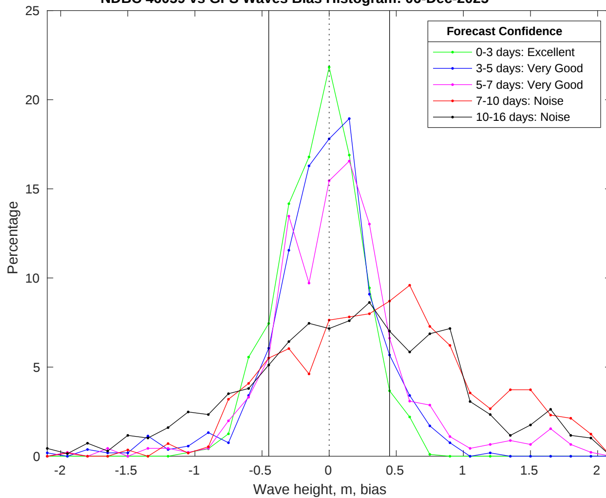
NDBC 46059 vs GFS Waves Bias Histogram: 06-Dec-2025
