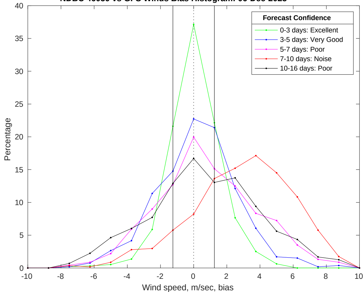
NDBC 46059 vs GFS Winds Bias Histogram: 06-Dec-2025
