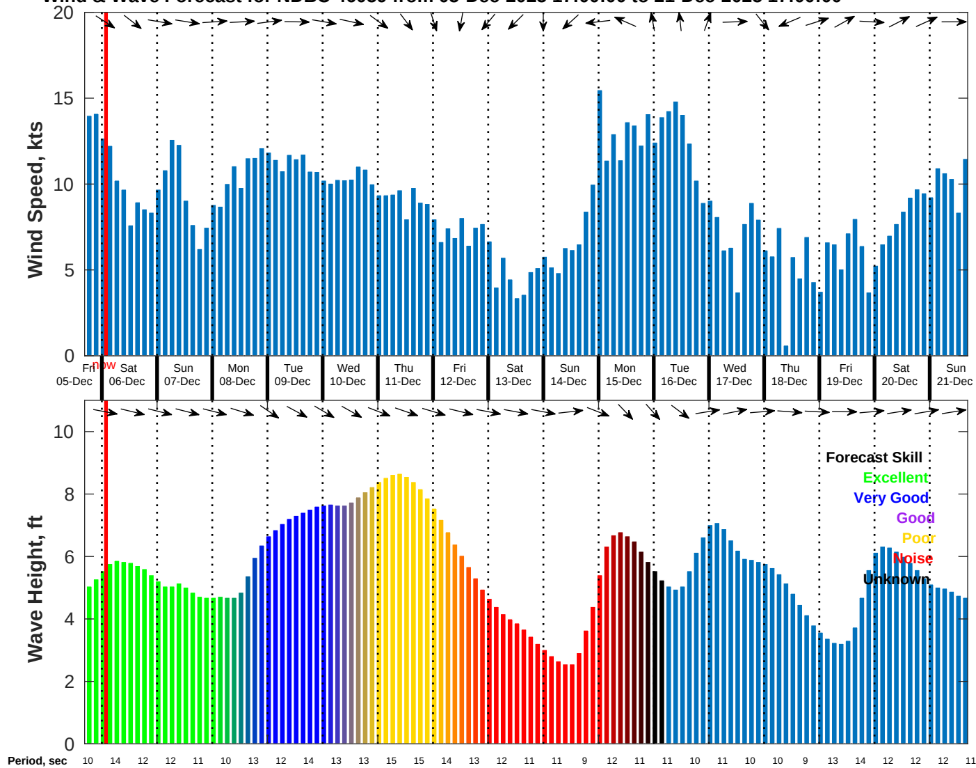
Wind & Wave Forecast for NDBC 46059 from 05-Dec-2025 17:00:00 to 21-Dec-2025 17:00:00
