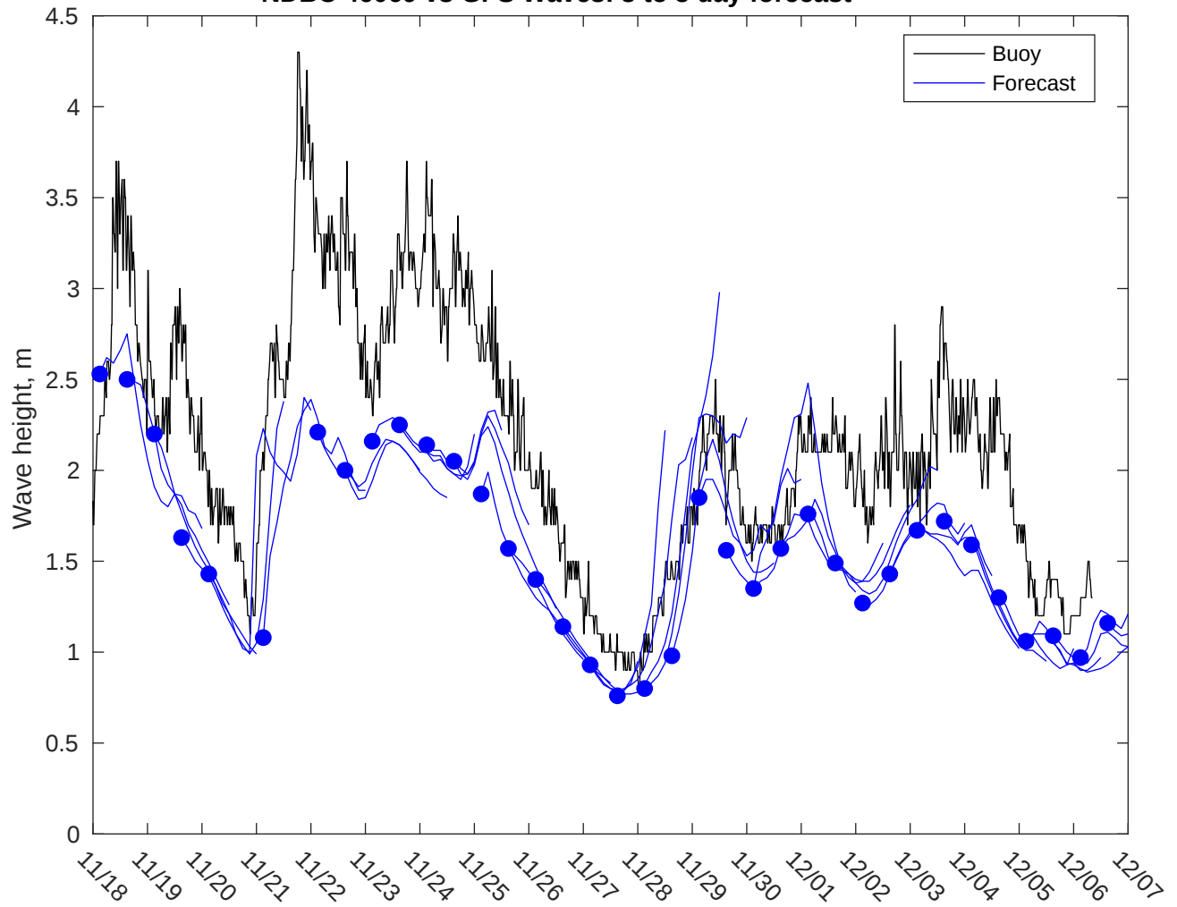
NDBC 46069 vs GFS Waves: 3 to 5 day forecast
