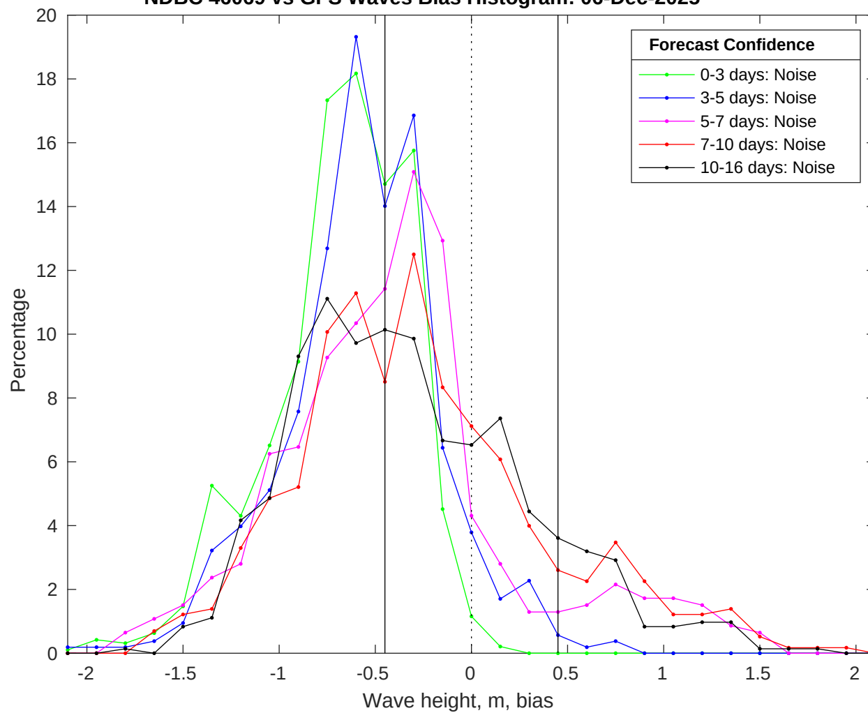
NDBC 46069 vs GFS Waves Bias Histogram: 06-Dec-2025
