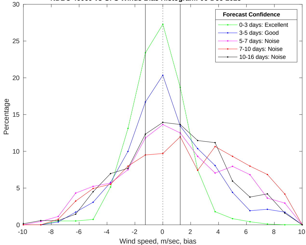
NDBC 46069 vs GFS Winds Bias Histogram: 06-Dec-2025
