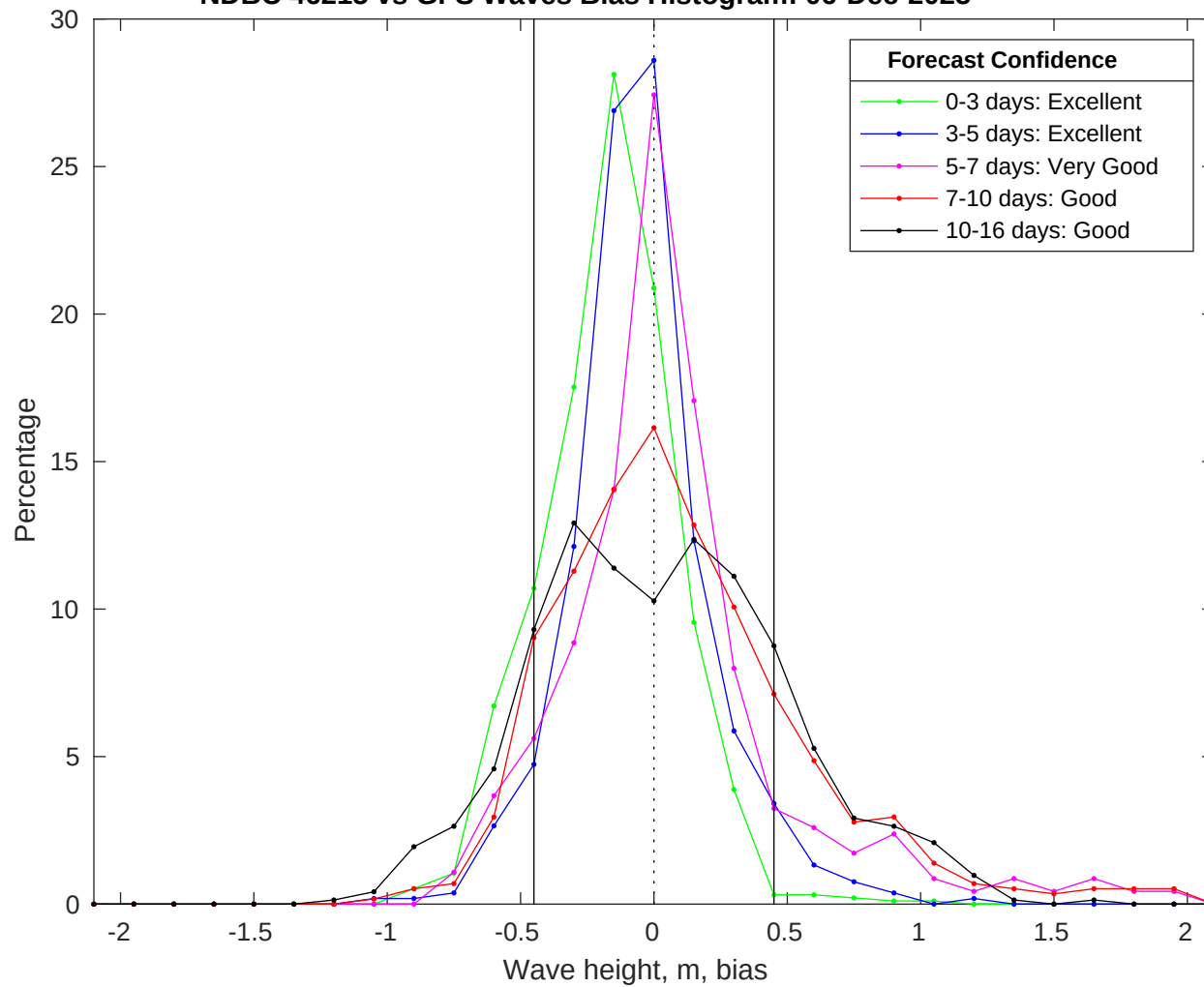
NDBC 46215 vs GFS Waves Bias Histogram: 06-Dec-2025
