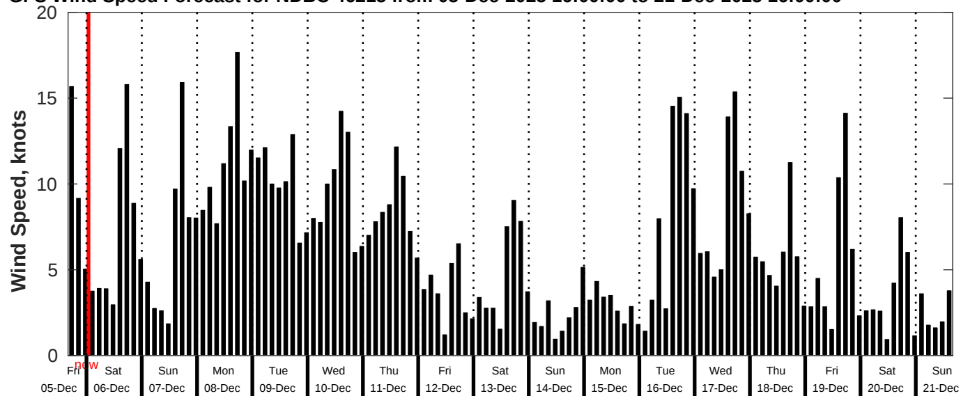
GFS Wind Speed Forecast for NDBC 46215 from 05-Dec-2025 16:00:00 to 21-Dec-2025 16:00:00
