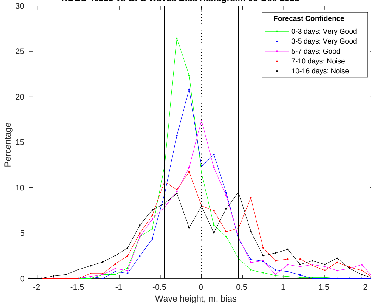
NDBC 46259 vs GFS Waves Bias Histogram: 06-Dec-2025
