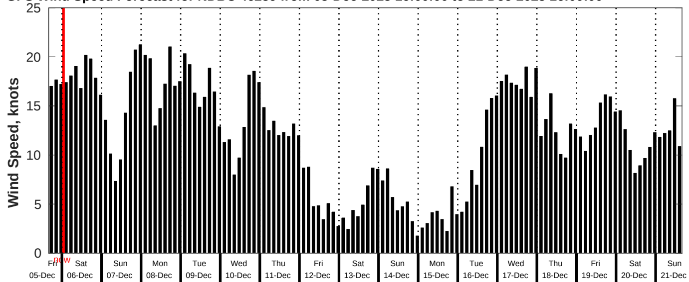
GFS Wind Speed Forecast for NDBC 46259 from 05-Dec-2025 16:00:00 to 21-Dec-2025 16:00:00
