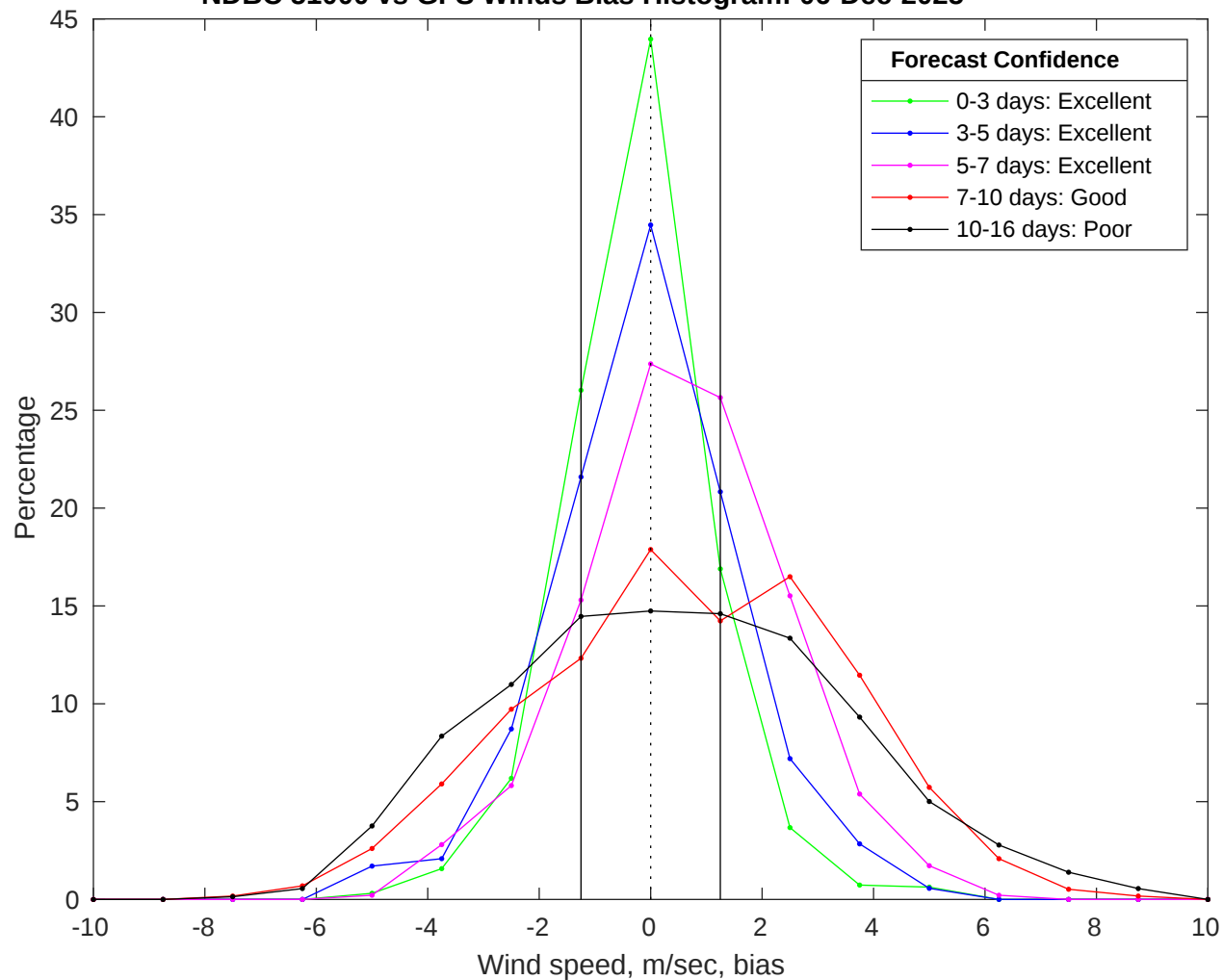
NDBC 51000 vs GFS Winds Bias Histogram: 06-Dec-2025
