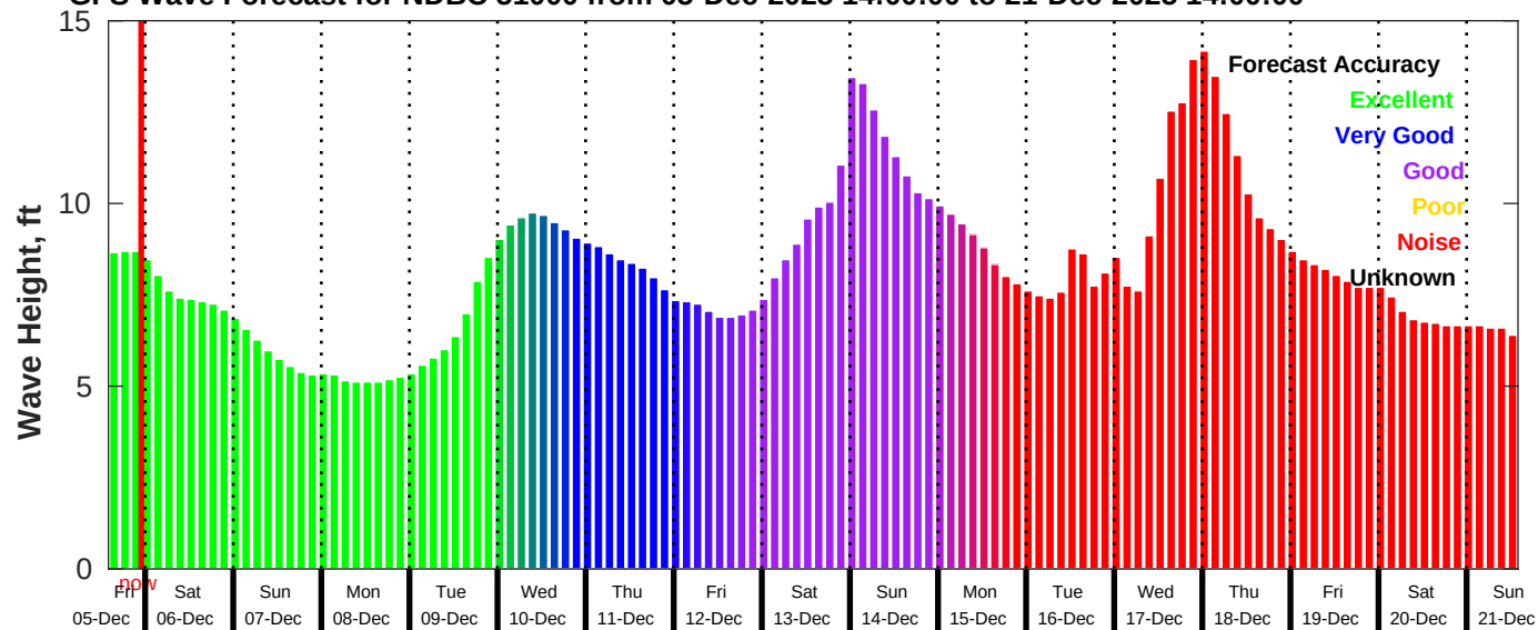
GFS Wave Forecast for NDBC 51000 from 05-Dec-2025 14:00:00 to 21-Dec-2025 14:00:00
