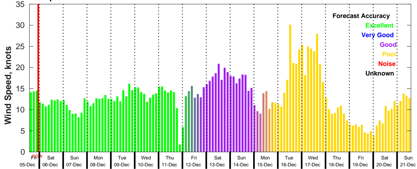
GFS Wind Speed Forecast for NDBC 51000 from 05-Dec-2025 14:00:00 to 21-Dec-2025 14:00:00
