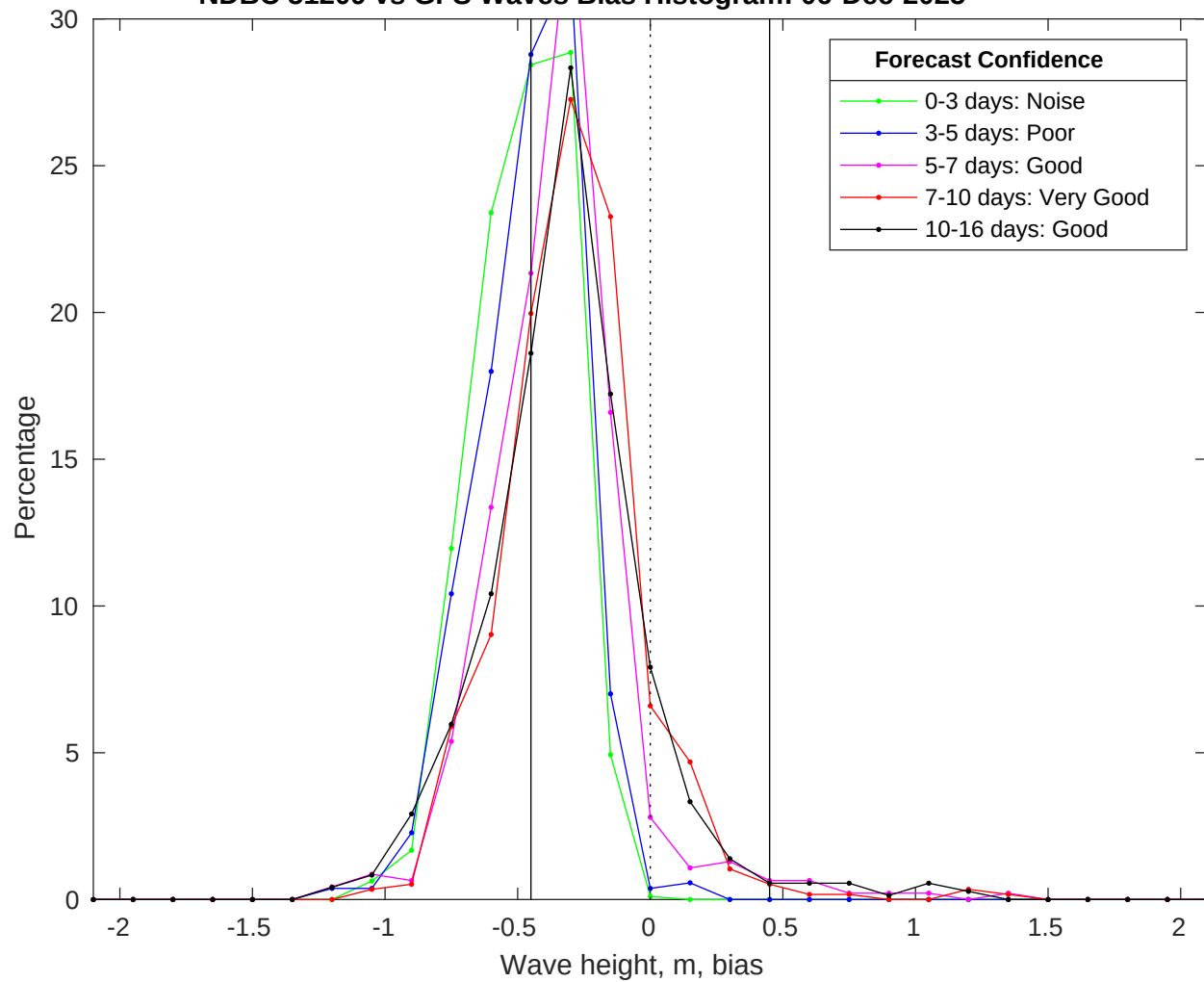
NDBC 51209 vs GFS Waves Bias Histogram: 06-Dec-2025
