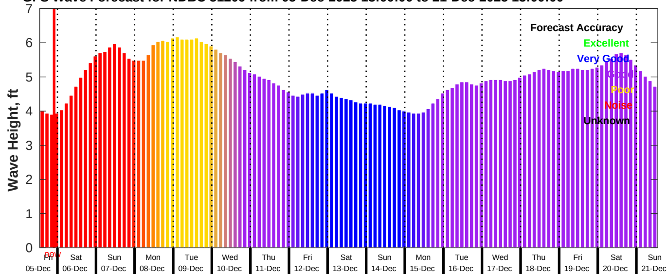
GFS Wave Forecast for NDBC 51209 from 05-Dec-2025 13:00:00 to 21-Dec-2025 13:00:00
