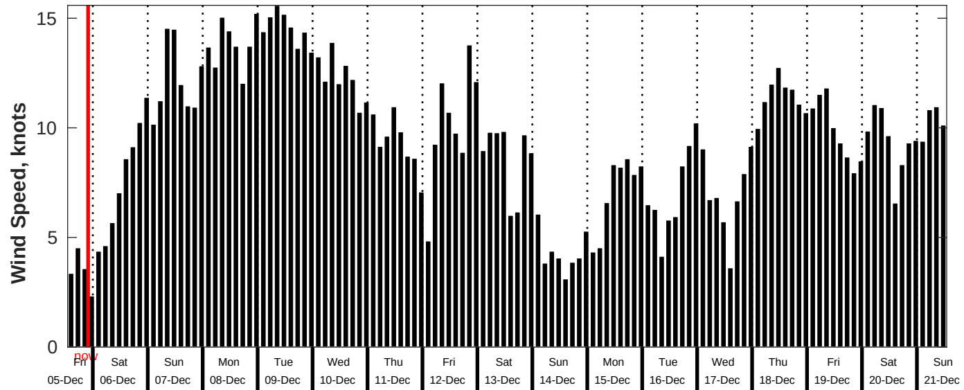
GFS Wind Speed Forecast for NDBC 51209 from 05-Dec-2025 13:00:00 to 21-Dec-2025 13:00:00
