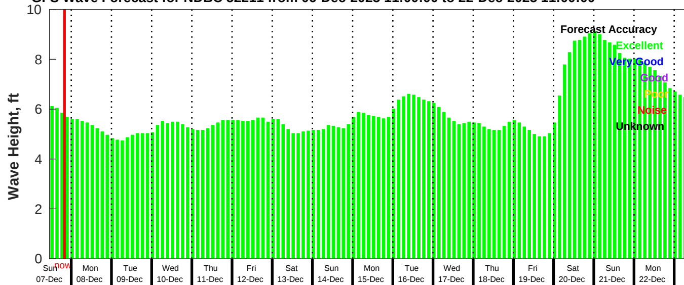
GFS Wave Forecast for NDBC 52211 from 06-Dec-2025 11:00:00 to 22-Dec-2025 11:00:00
