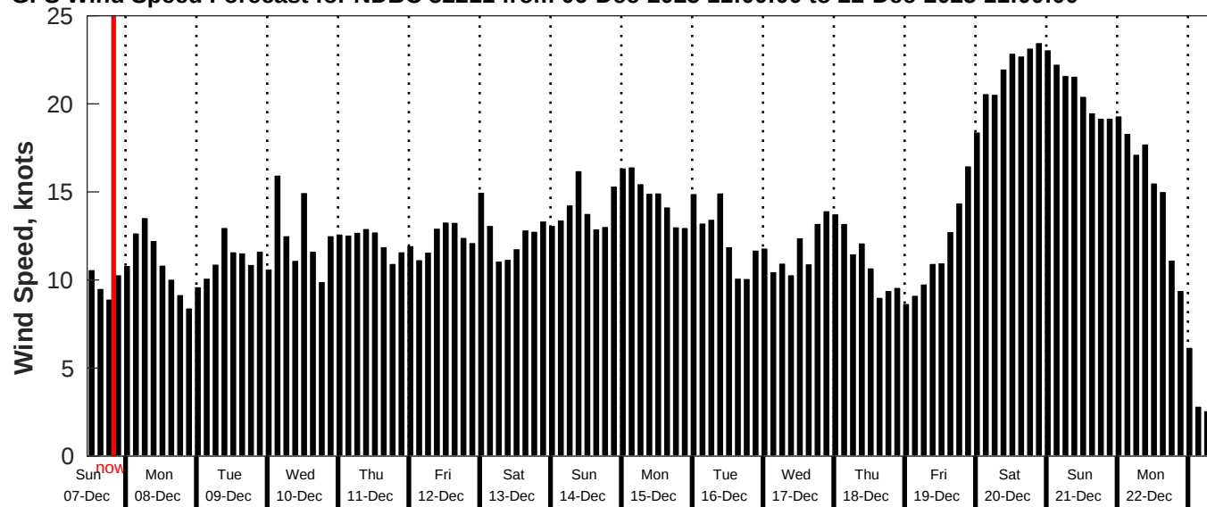
GFS Wind Speed Forecast for NDBC 52211 from 06-Dec-2025 11:00:00 to 22-Dec-2025 11:00:00
