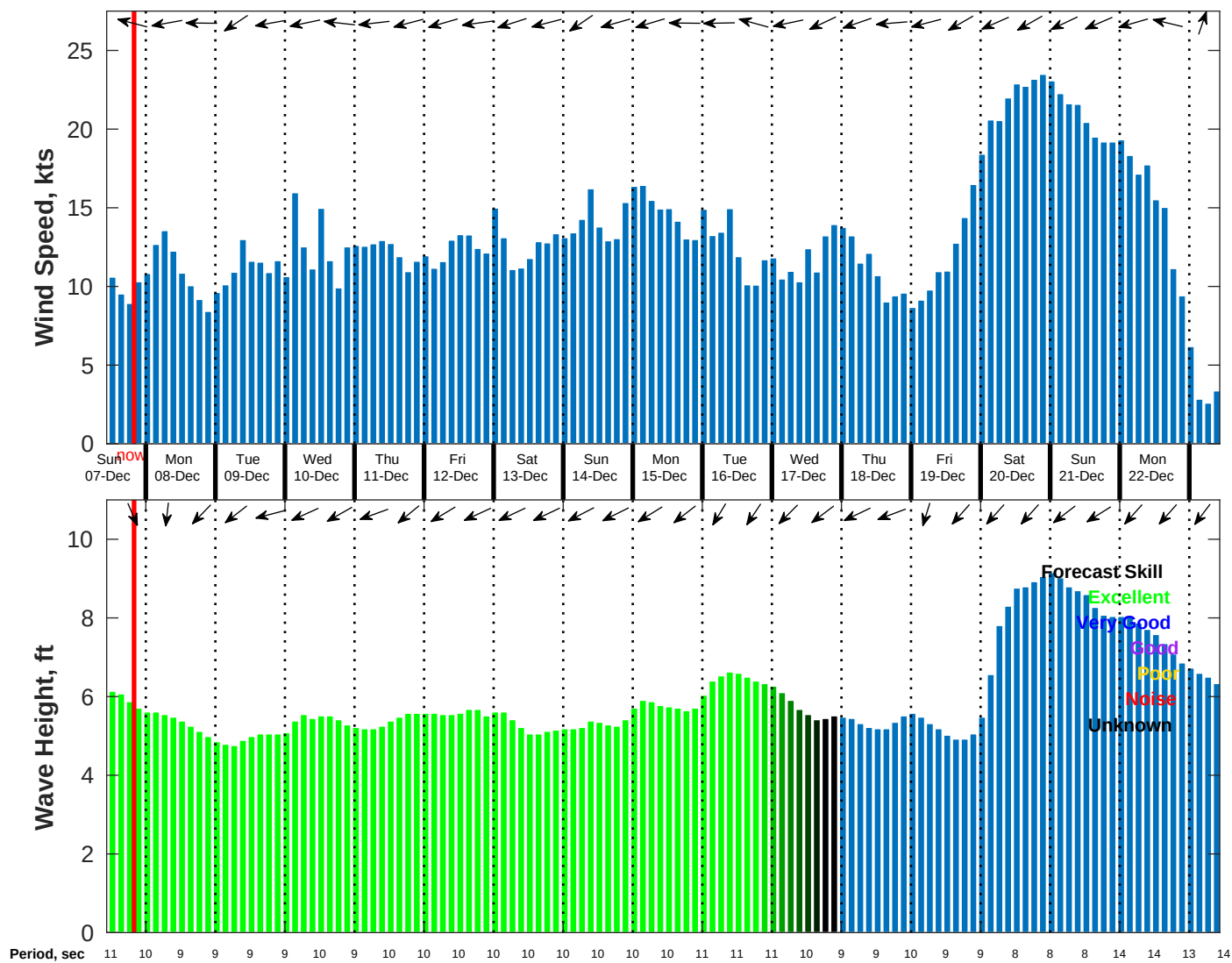
Wind & Wave Forecast for NDBC 52211 from 06-Dec-2025 11:00:00 to 22-Dec-2025 11:00:00
