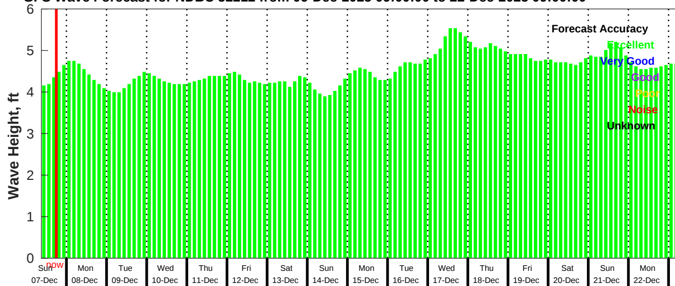
GFS Wave Forecast for NDBC 52212 from 06-Dec-2025 09:00:00 to 22-Dec-2025 09:00:00
