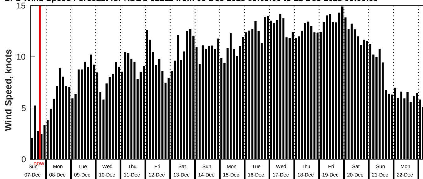
GFS Wind Speed Forecast for NDBC 52212 from 06-Dec-2025 09:00:00 to 22-Dec-2025 09:00:00
