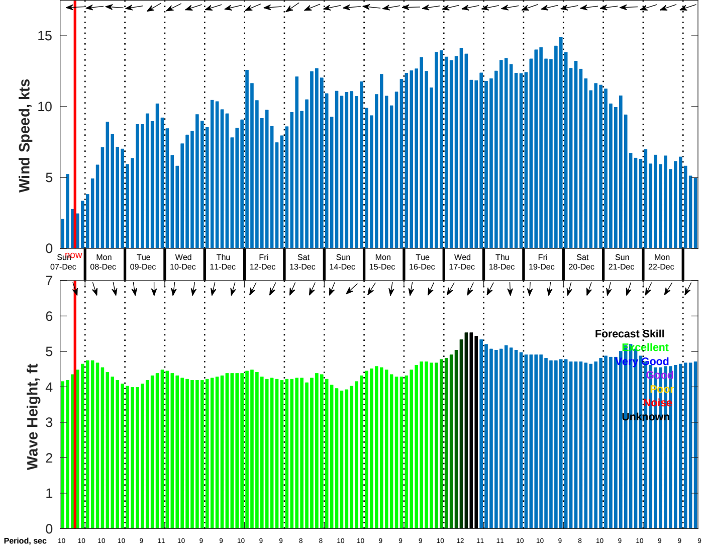
Wind & Wave Forecast for NDBC 52212 from 06-Dec-2025 09:00:00 to 22-Dec-2025 09:00:00
