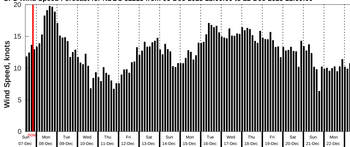
GFS Wind Speed Forecast for NDBC 52213 from 06-Dec-2025 11:00:00 to 22-Dec-2025 11:00:00
