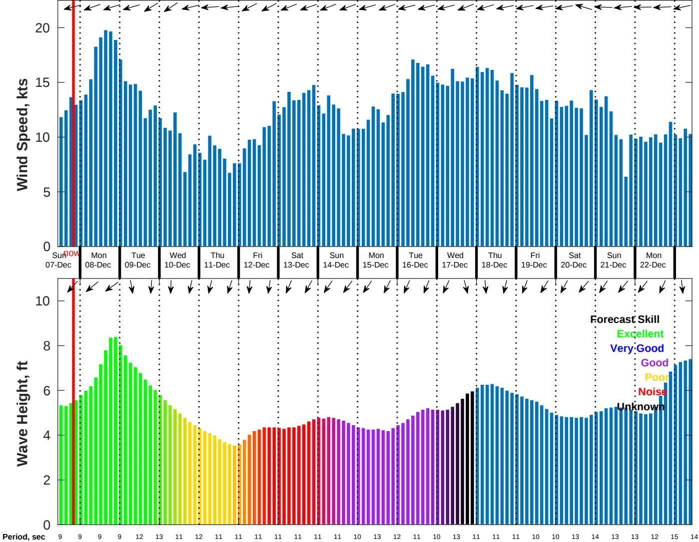
Wind & Wave Forecast for NDBC 52213 from 06-Dec-2025 11:00:00 to 22-Dec-2025 11:00:00
