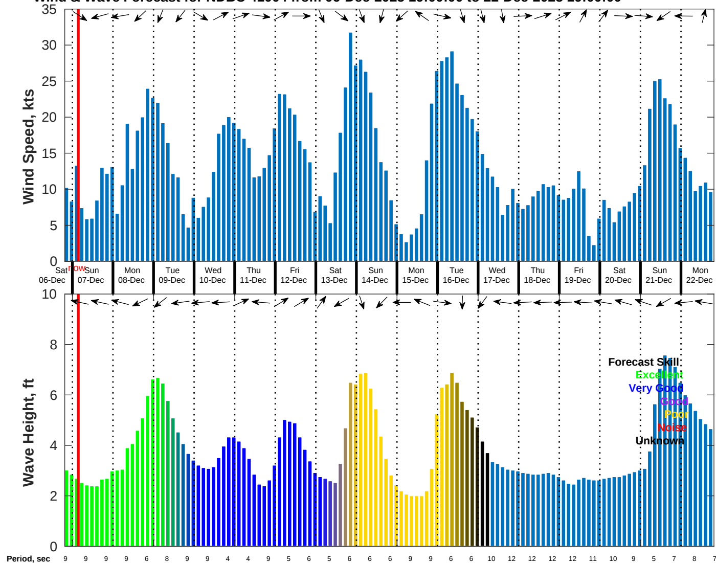
Wind & Wave Forecast for NDBC 41004 from 06-Dec-2025 19:00:00 to 22-Dec-2025 19:00:00
